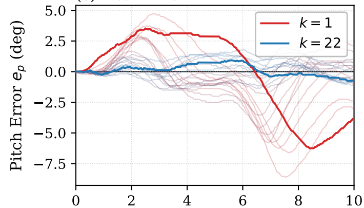
(c) Pitch Error
