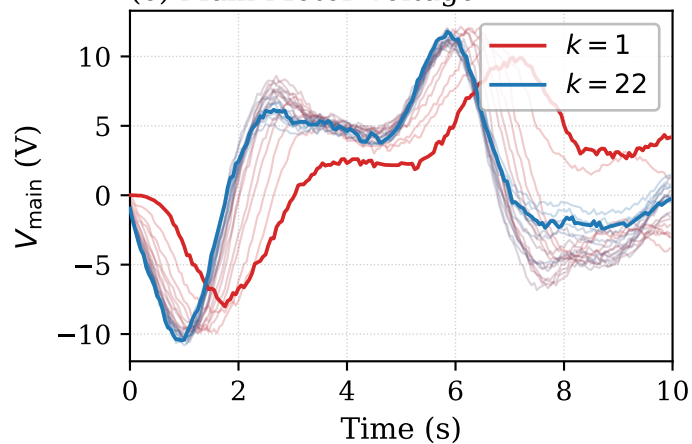
(e) Main Motor Voltage
