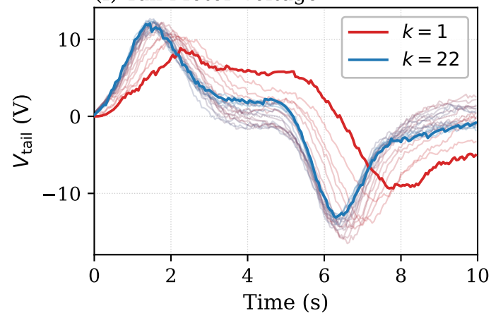
(f) Tail Motor Voltage
