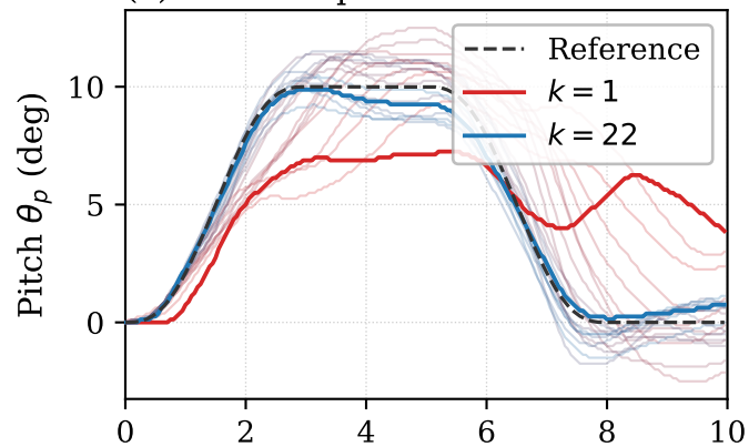
(a) Pitch Output
