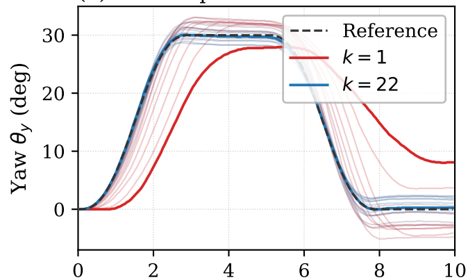
(b) Yaw Output
